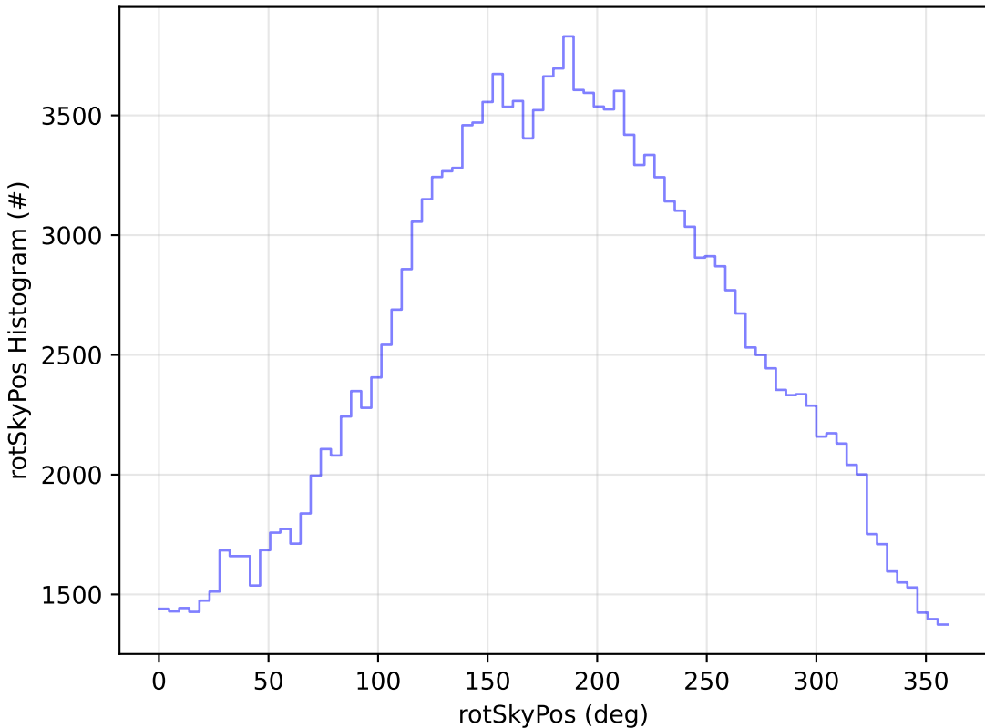
start_date_do-180v3.4_10yrs All sky g band: rotSkyPos Histogram
