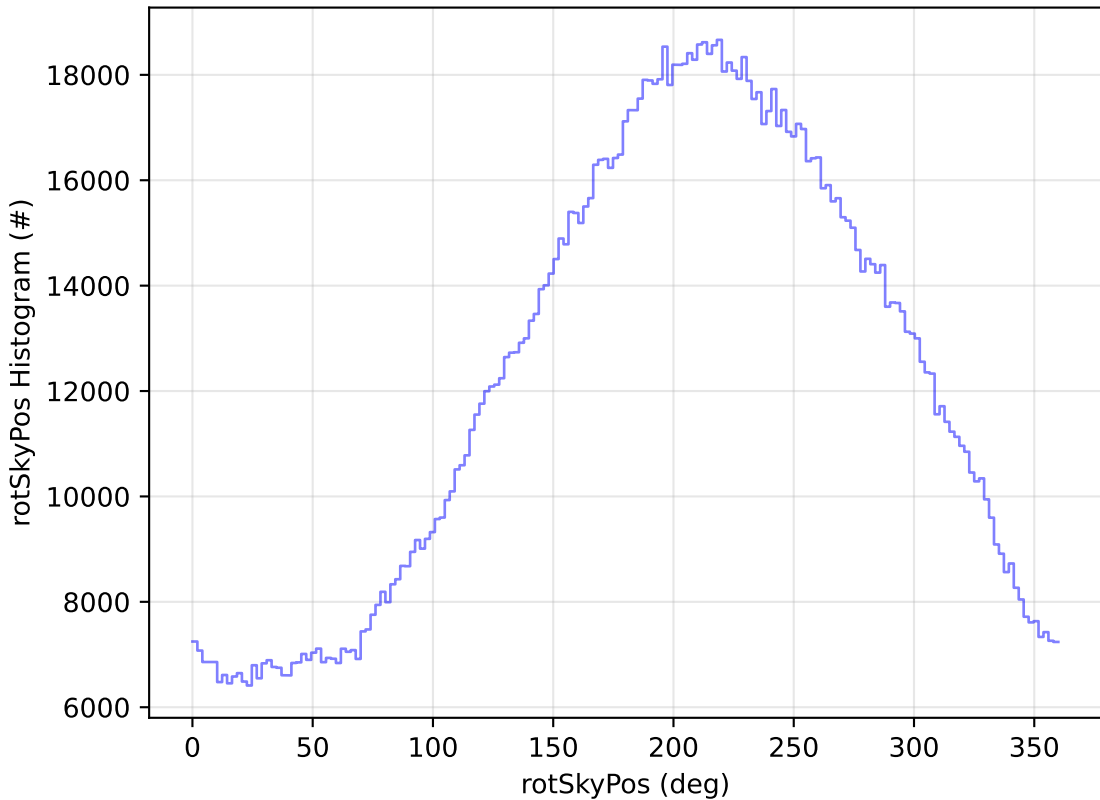
start_date_do-180v3.4_10yrs All sky all bands: rotSkyPos Histogram
