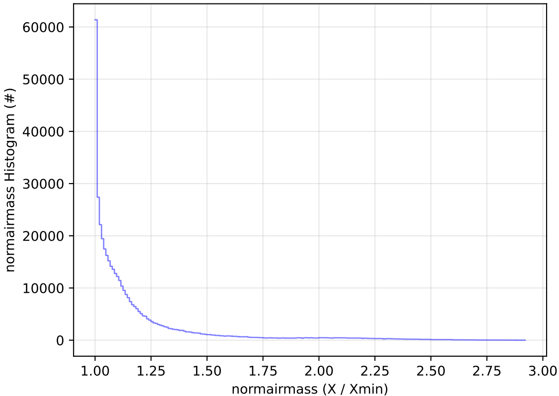
start_date_do-180v3.4_10yrs WFD z band: normairmass Histogram
