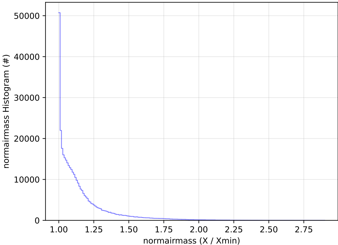
start_date_do-180v3.4_10yrs WFD y band: normairmass Histogram
