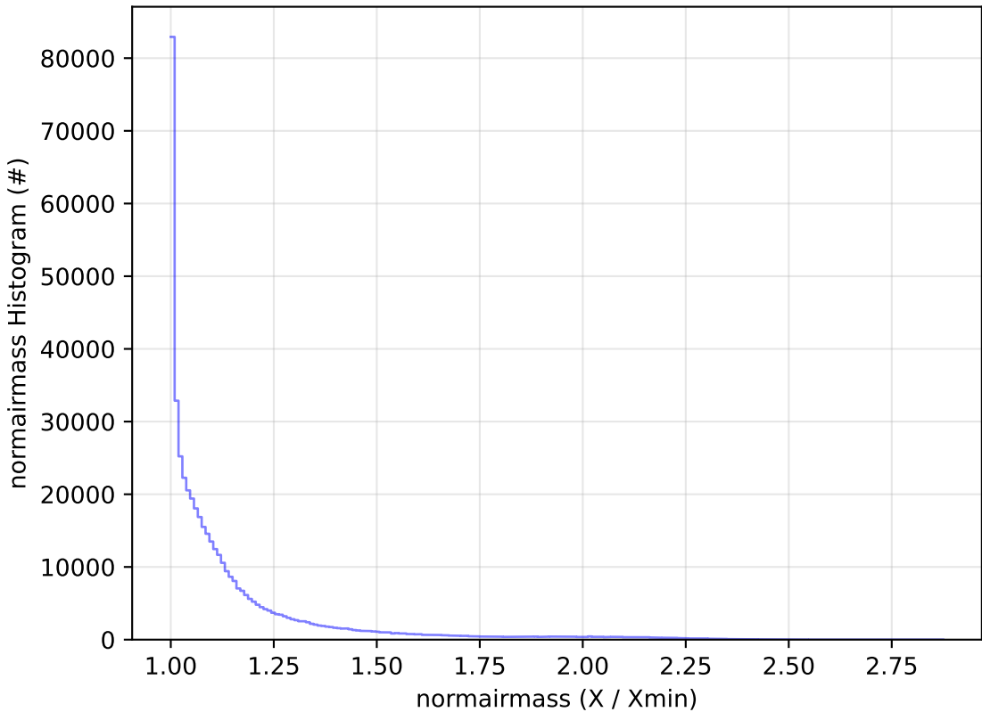
start_date_do-180v3.4_10yrs WFD r band: normairmass Histogram
