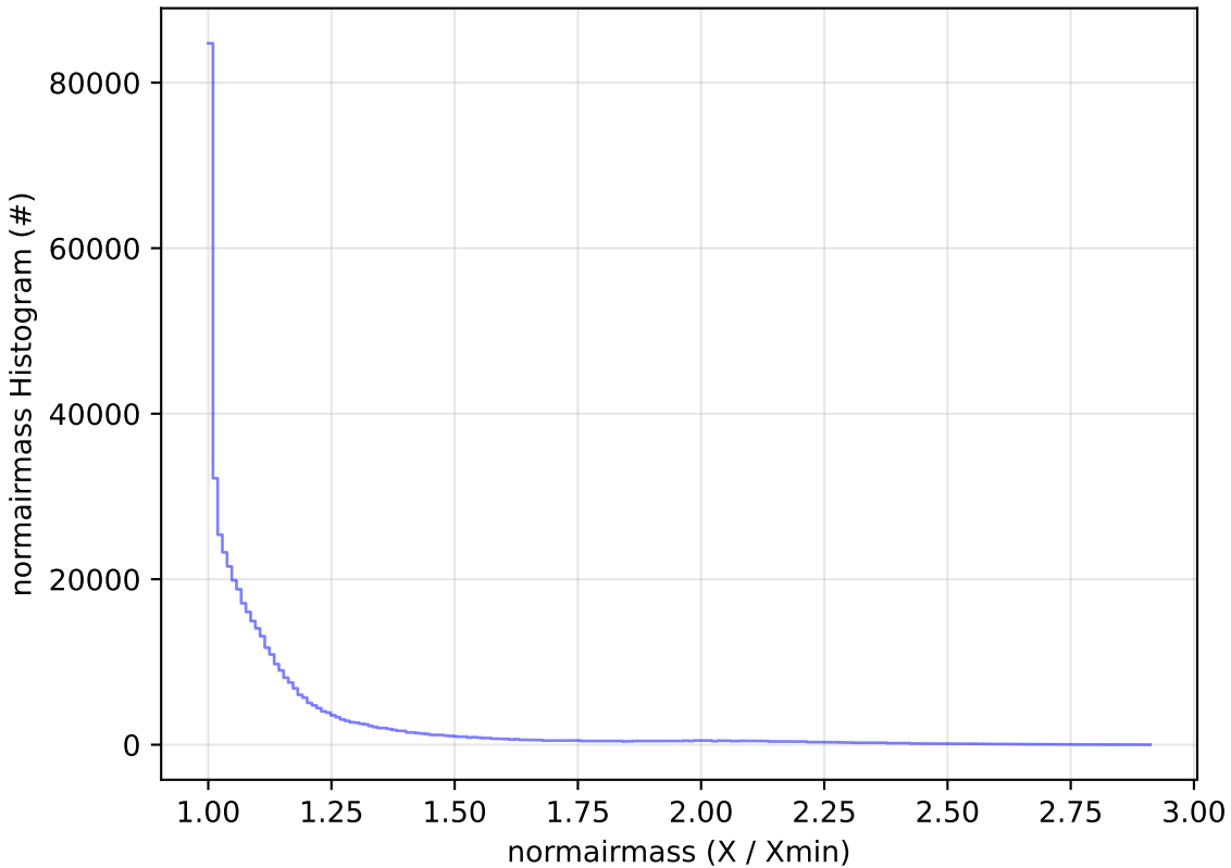
start_date_do-180v3.4_10yrs WFD i band: normairmass Histogram
