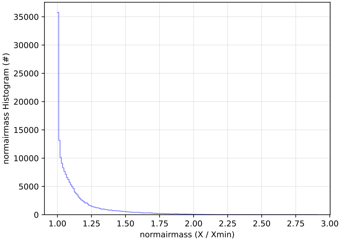
start_date_do-180v3.4_10yrs WFD g band: normairmass Histogram
