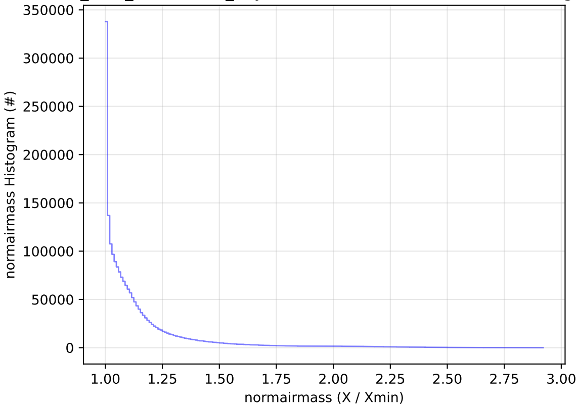
start_date_do-180v3.4_10yrs WFD all bands: normairmass Histogram
