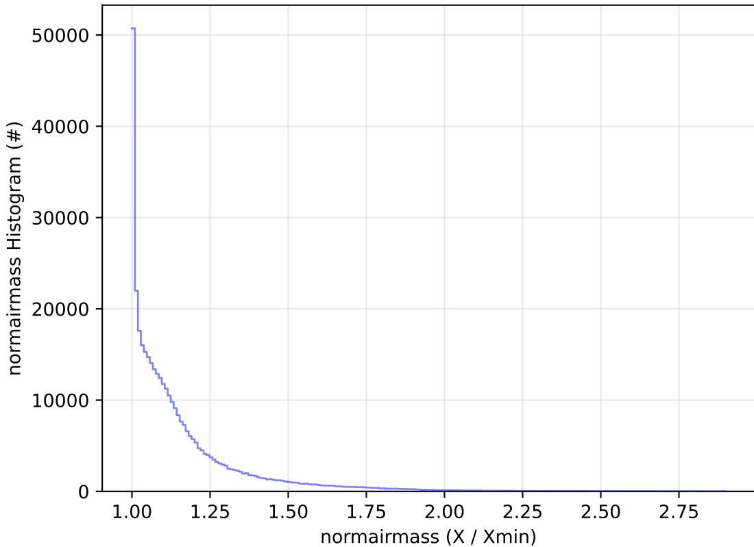
start_date_do-180v3.4_10yrs All sky y band: normairmass Histogram
