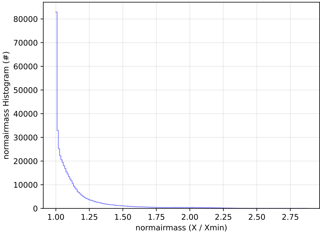
start_date_do-180v3.4_10yrs All sky r band: normairmass Histogram
