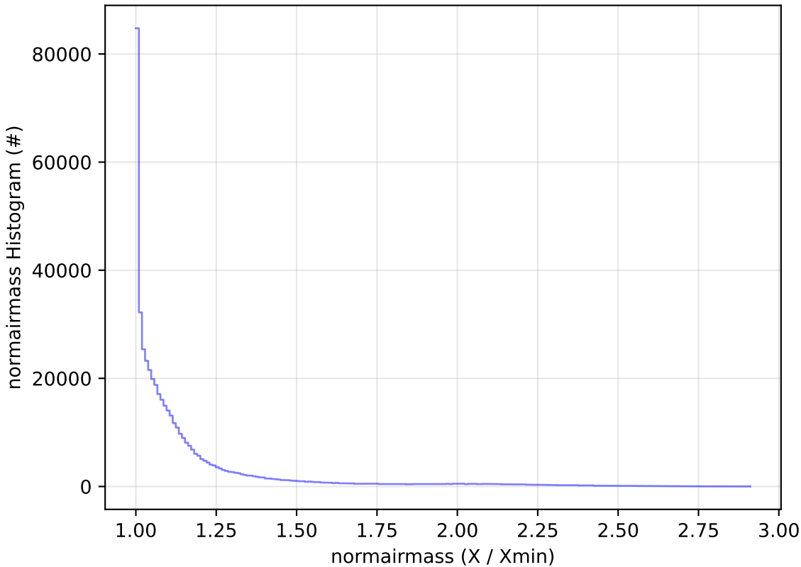
start_date_do-180v3.4_10yrs All sky i band: normairmass Histogram
