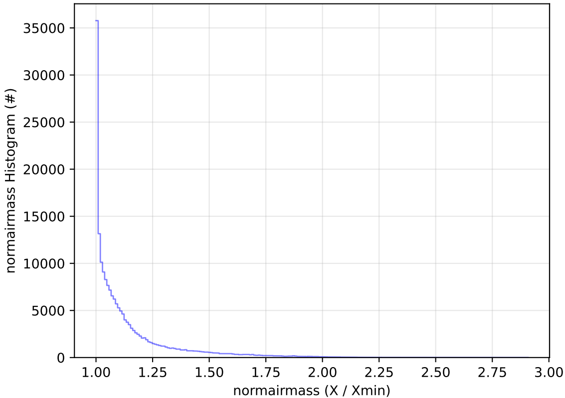
start_date_do-180v3.4_10yrs All sky g band: normairmass Histogram
