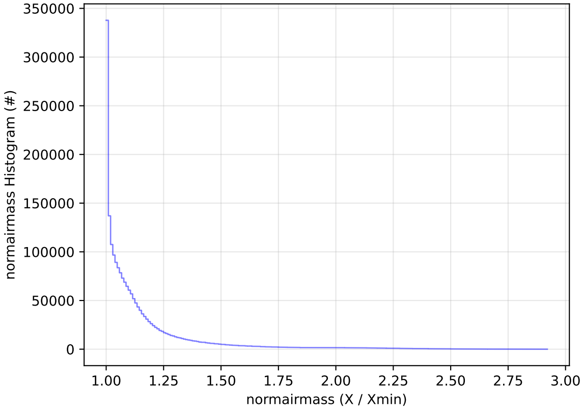
start_date_do-180v3.4_10yrs All sky all bands: normairmass Histogram
