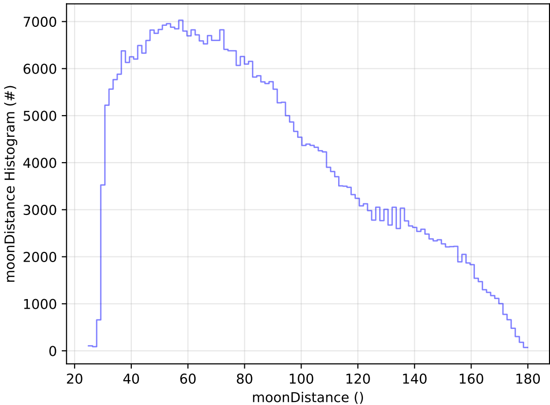
start_date_do-180v3.4_10yrs WFD z band: moonDistance Histogram
