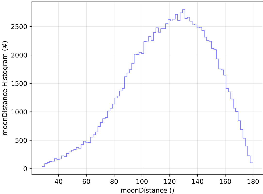
start_date_do-180v3.4_10yrs WFD u band: moonDistance Histogram
