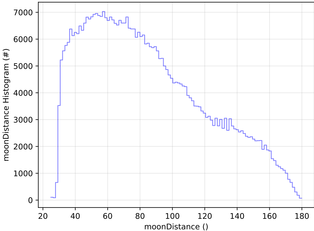
start_date_do-180v3.4_10yrs All sky z band: moonDistance Histogram
