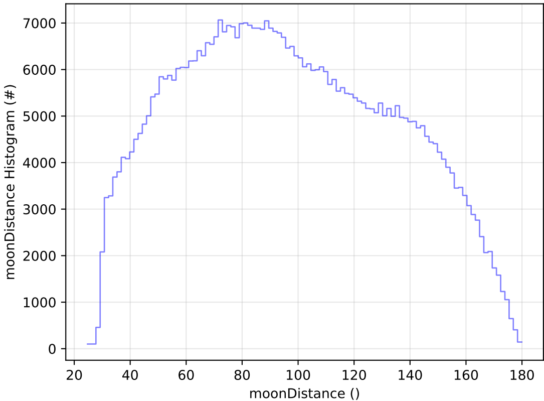
start_date_do-180v3.4_10yrs All sky i band: moonDistance Histogram
