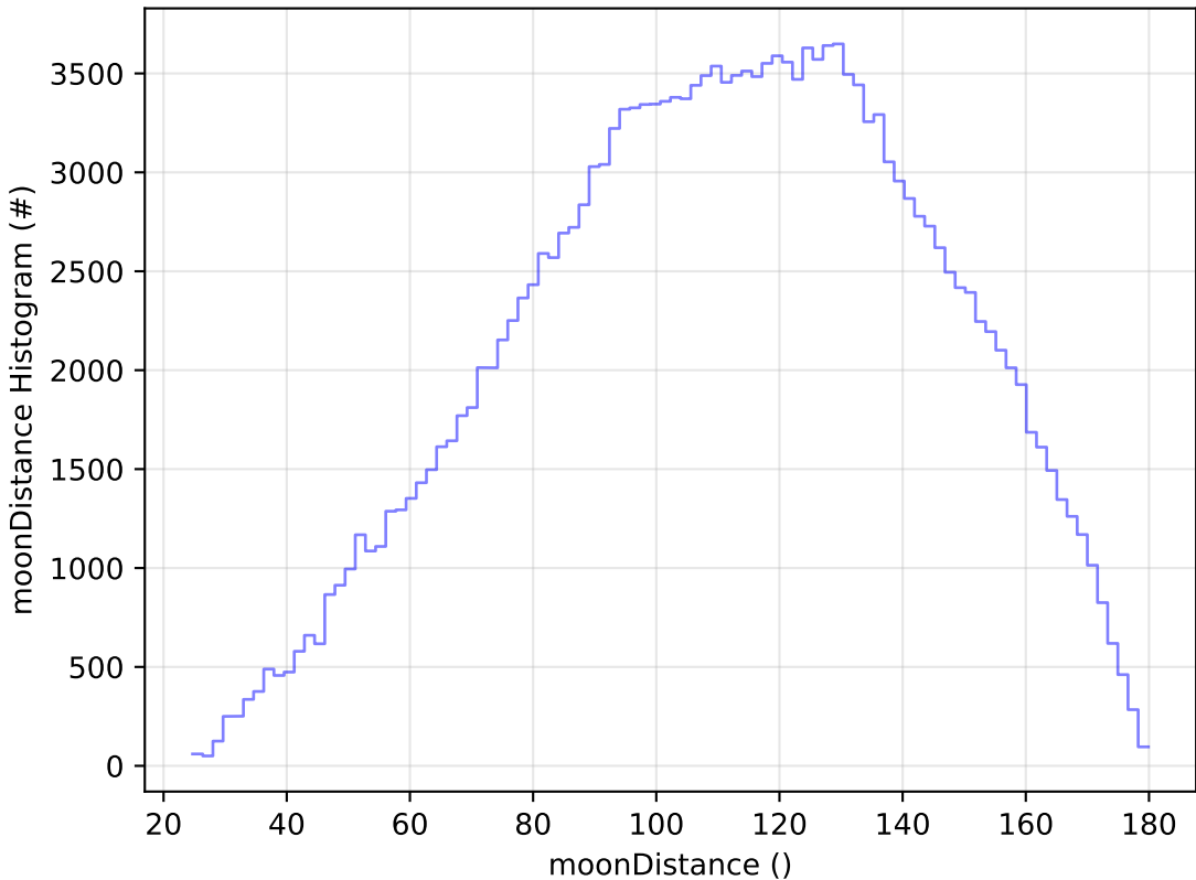
start_date_do-180v3.4_10yrs All sky g band: moonDistance Histogram
