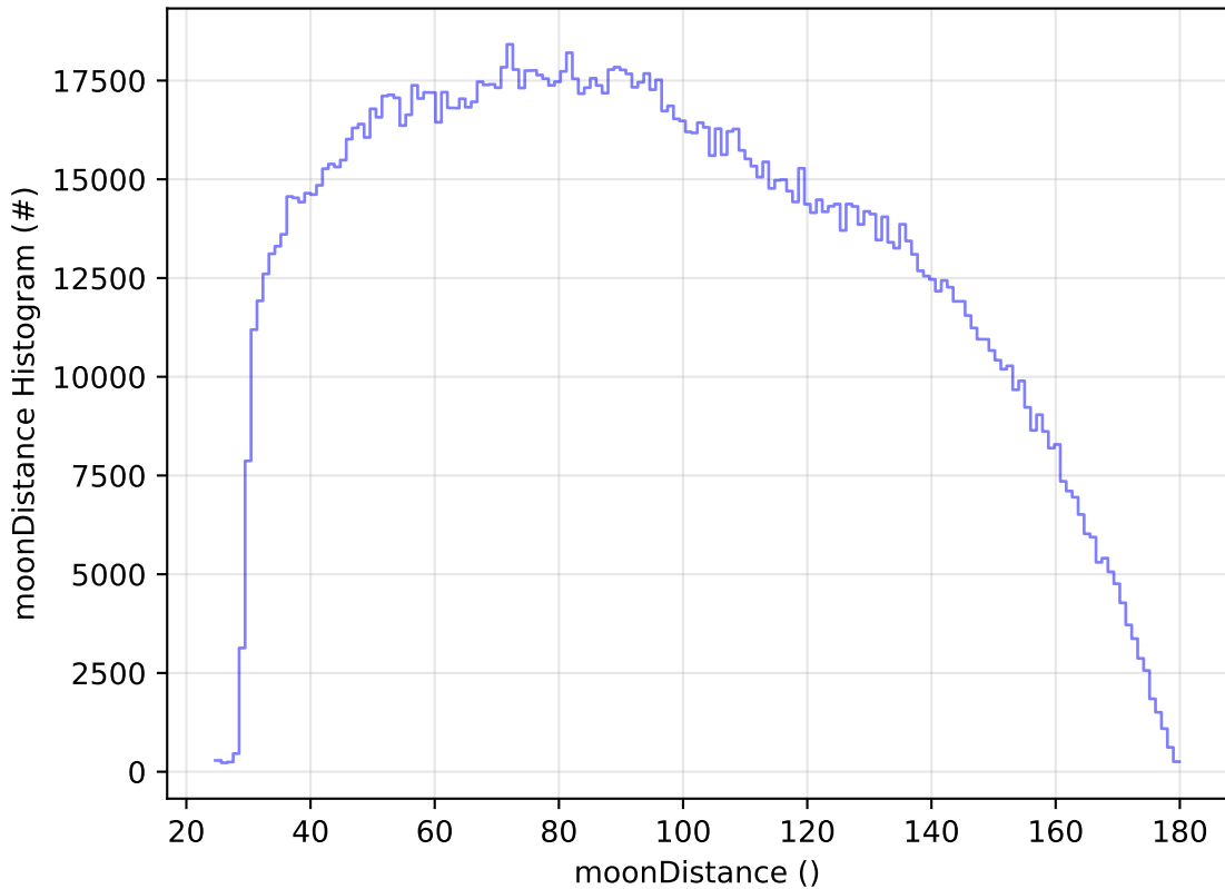
start_date_do-180v3.4_10yrs All sky all bands: moonDistance Histogram
