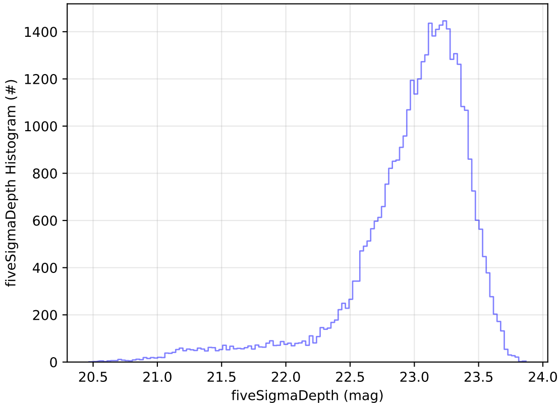
start_date_do-180v3.4_10yrs Yr 1 z band: fiveSigmaDepth Histogram
