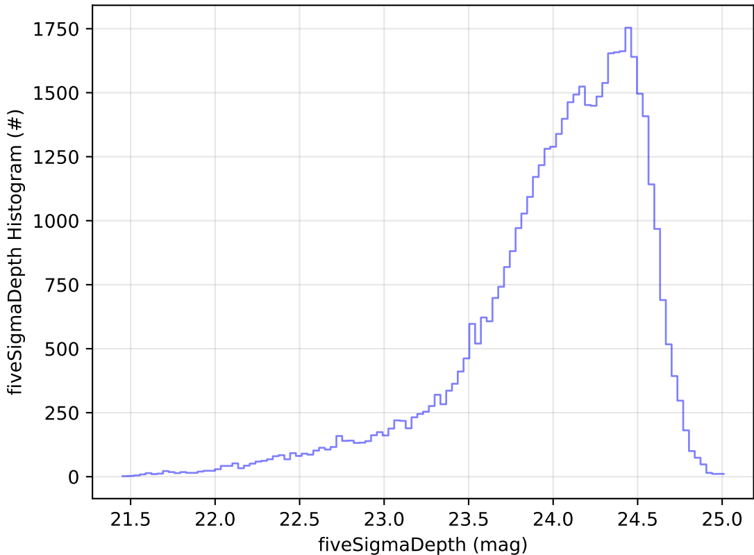
start_date_do-180v3.4_10yrs Yr 1 r band: fiveSigmaDepth Histogram
