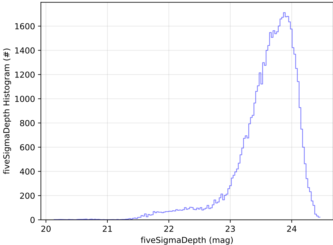
start_date_do-180v3.4_10yrs Yr 1 i band: fiveSigmaDepth Histogram
