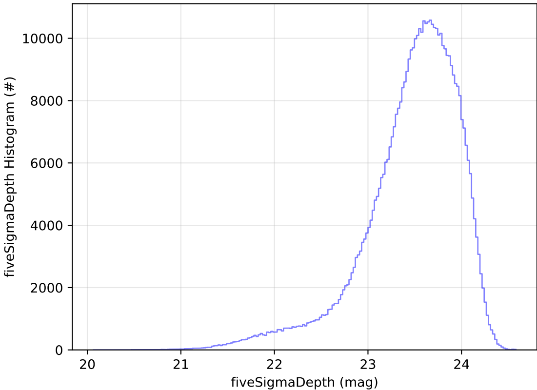
start_date_do-180v3.4_10yrs WFD i band: fiveSigmaDepth Histogram
