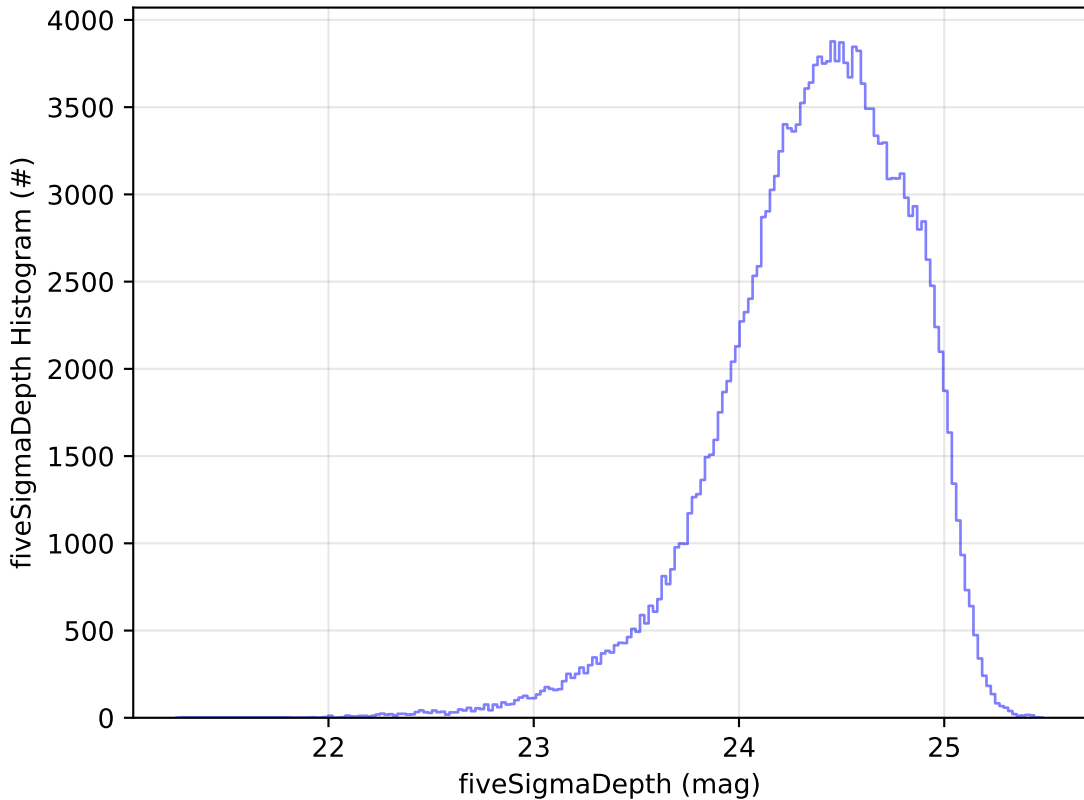
start_date_do-180v3.4_10yrs All sky g band: fiveSigmaDepth Histogram
