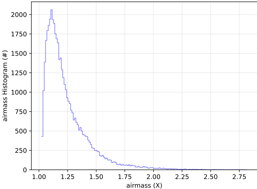
start_date_do-180v3.4_10yrs Yr 1 y band: airmass Histogram
