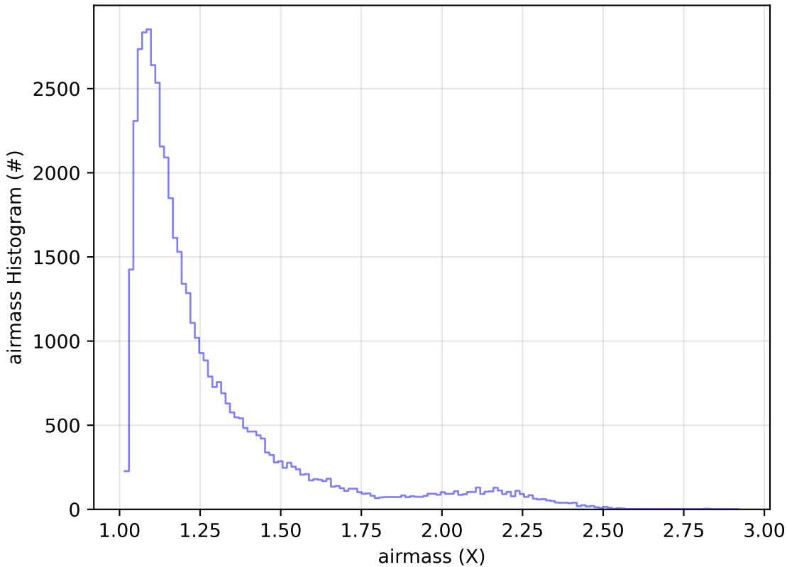
start_date_do-180v3.4_10yrs Yr 1 r band: airmass Histogram
