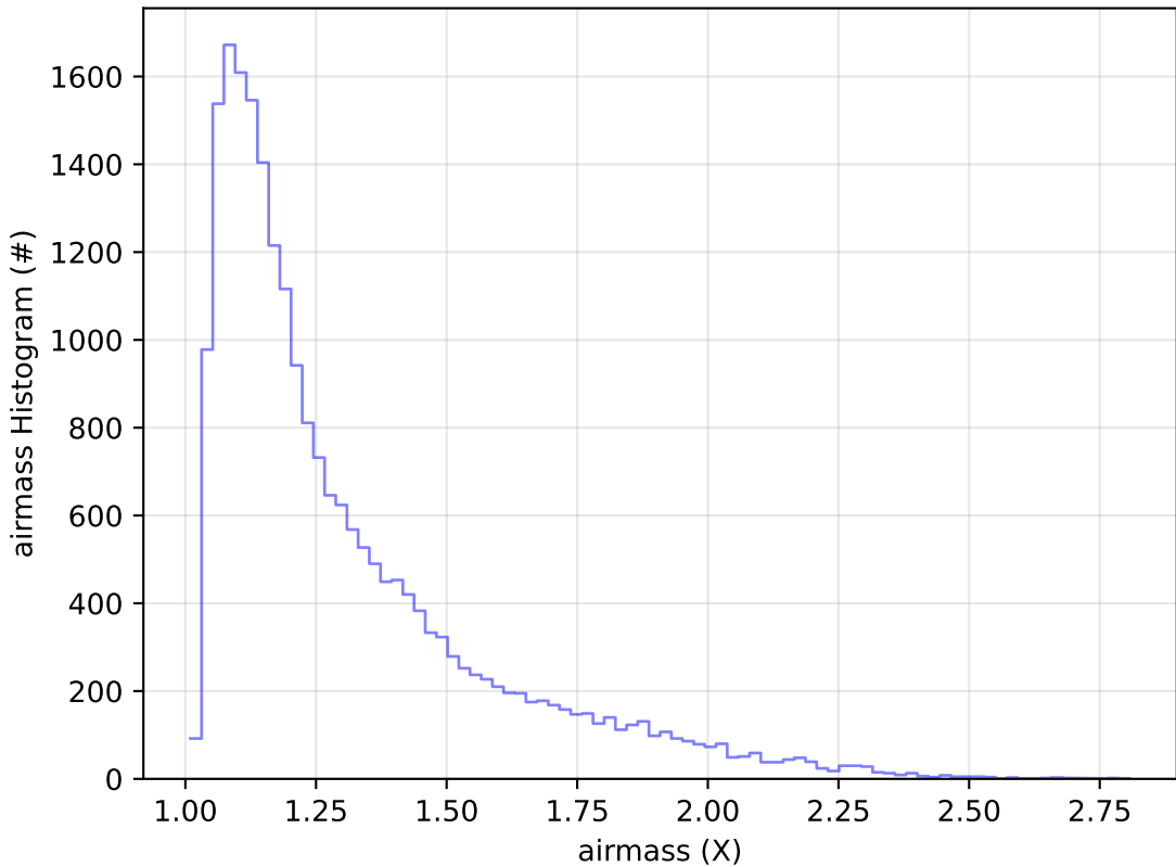
start_date_do-180v3.4_10yrs Yr 1 g band: airmass Histogram
