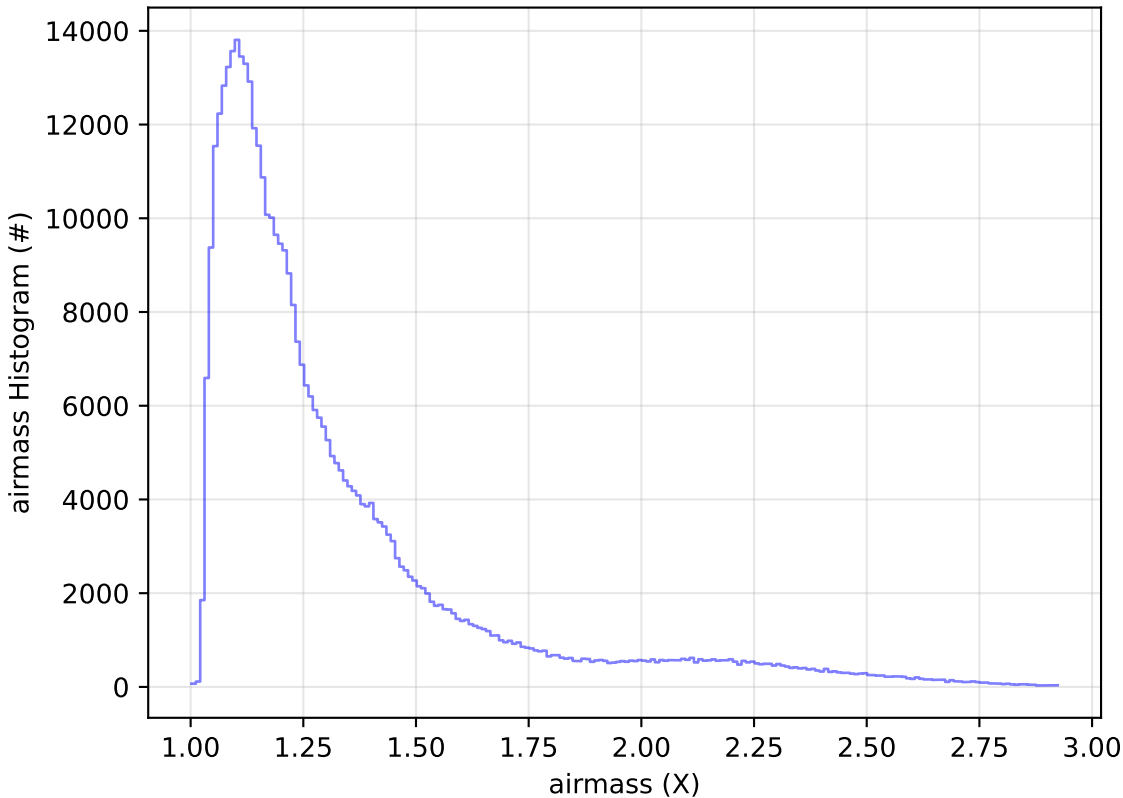
start_date_do-180v3.4_10yrs WFD z band: airmass Histogram
