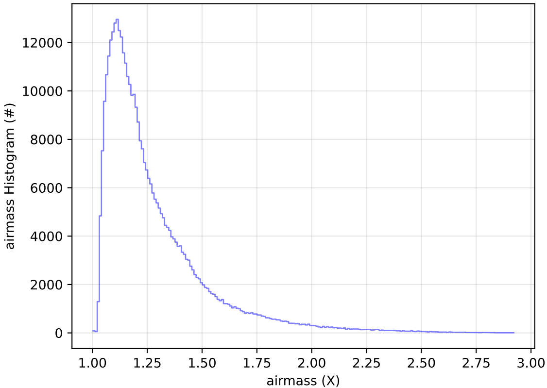
start_date_do-180v3.4_10yrs WFD y band: airmass Histogram
