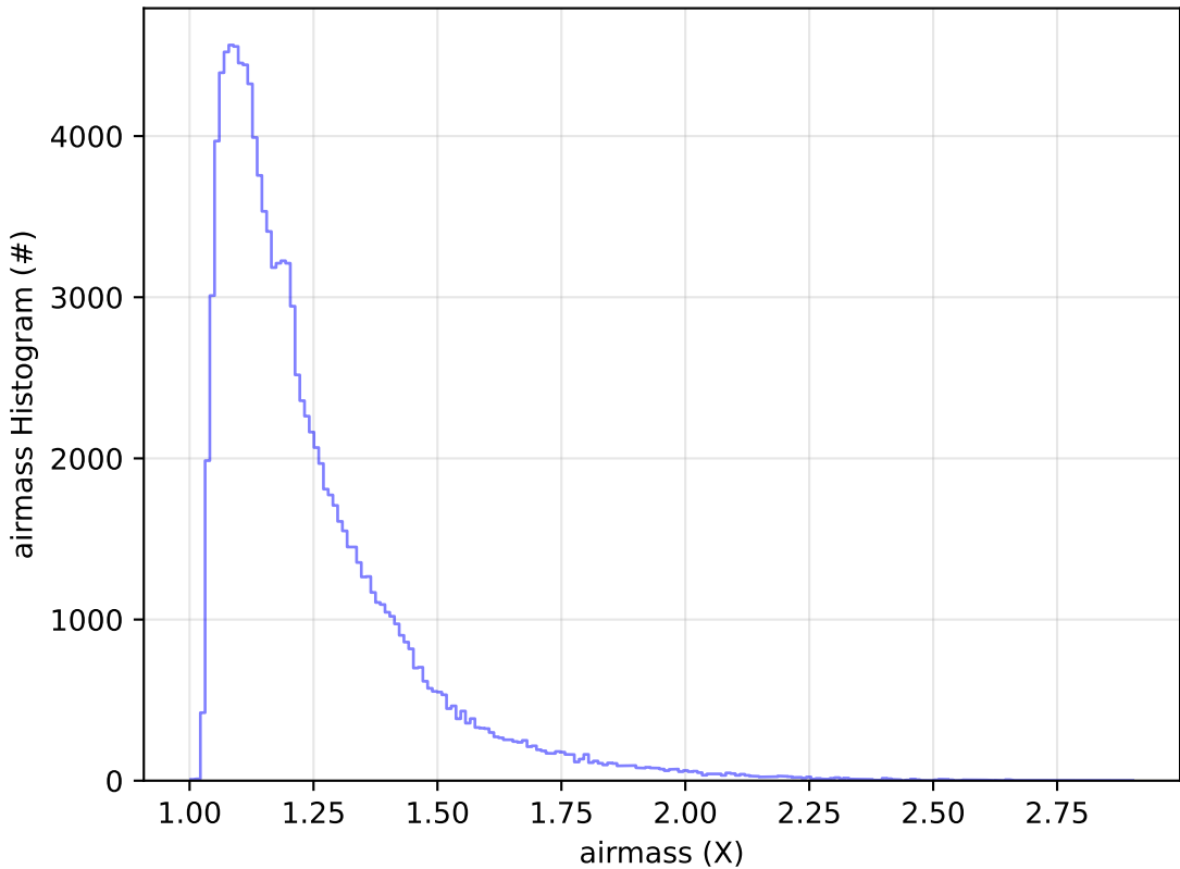
start_date_do-180v3.4_10yrs WFD u band: airmass Histogram
