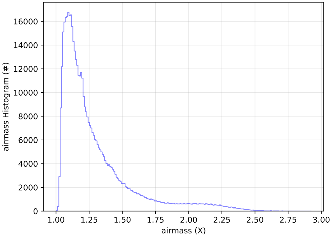
start_date_do-180v3.4_10yrs WFD r band: airmass Histogram
