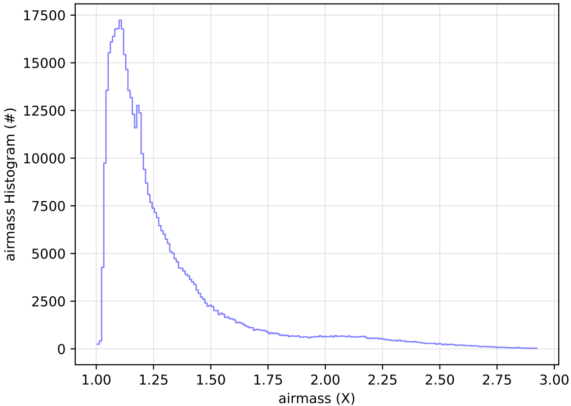
start_date_do-180v3.4_10yrs WFD i band: airmass Histogram
