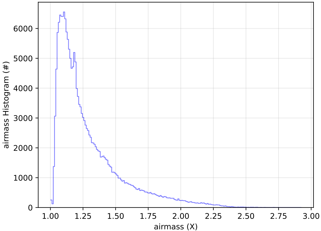
start_date_do-180v3.4_10yrs WFD g band: airmass Histogram
