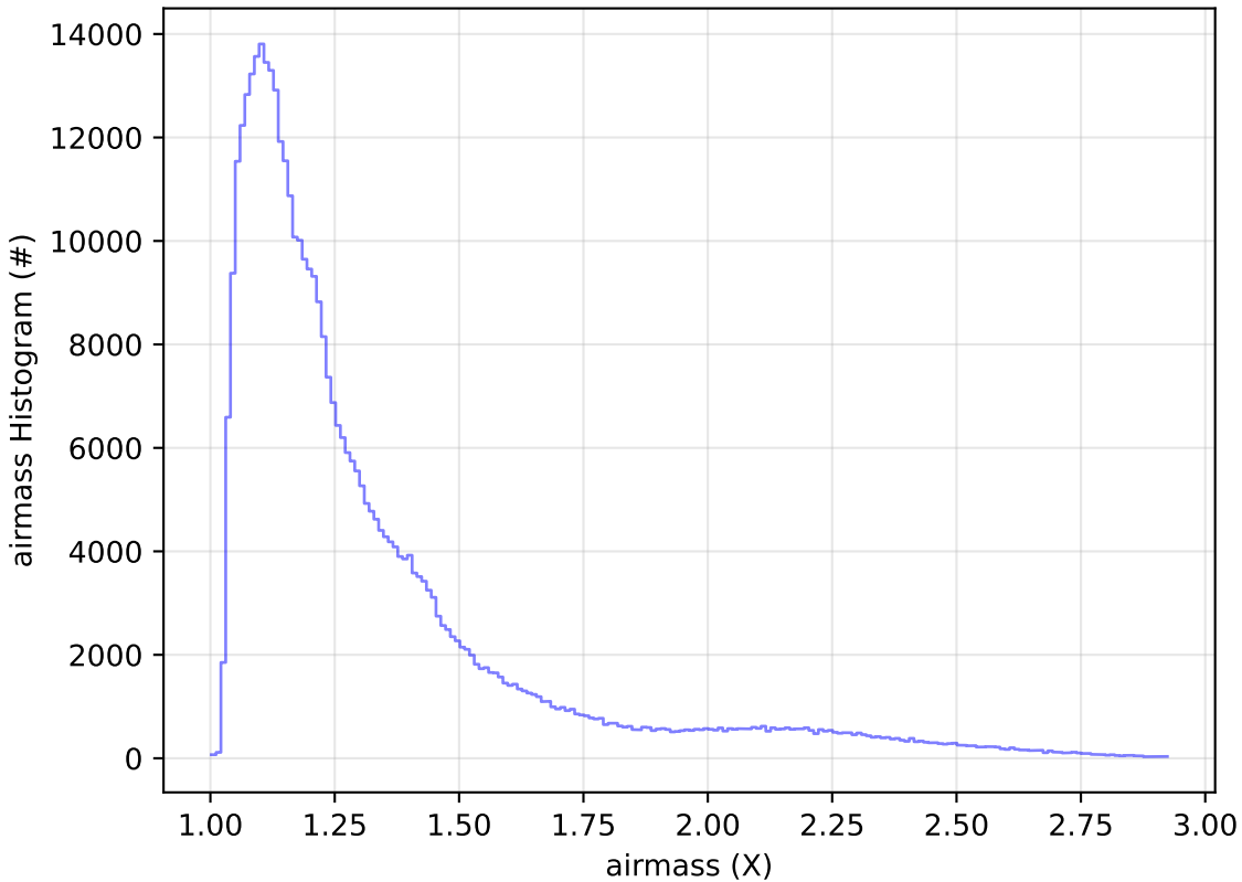
start_date_do-180v3.4_10yrs All sky z band: airmass Histogram
