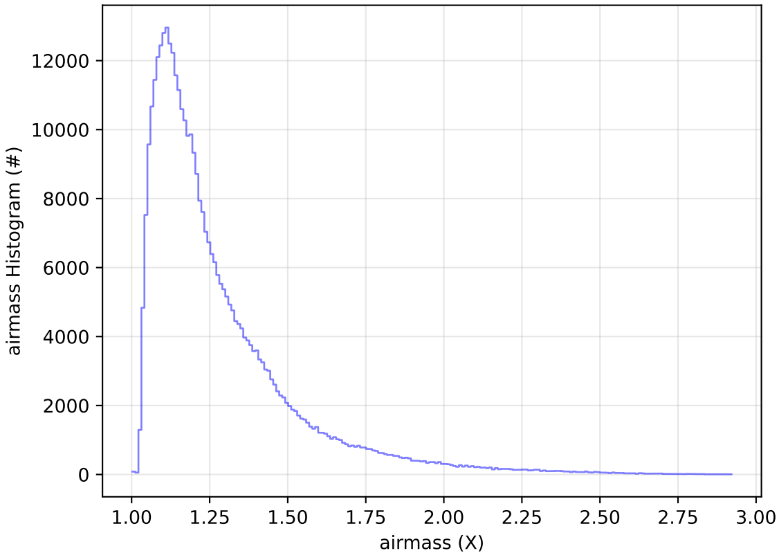
start_date_do-180v3.4_10yrs All sky y band: airmass Histogram
