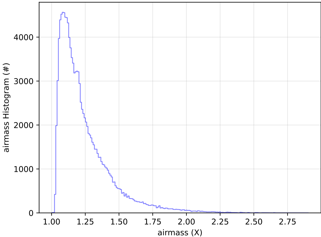
start_date_do-180v3.4_10yrs All sky u band: airmass Histogram
