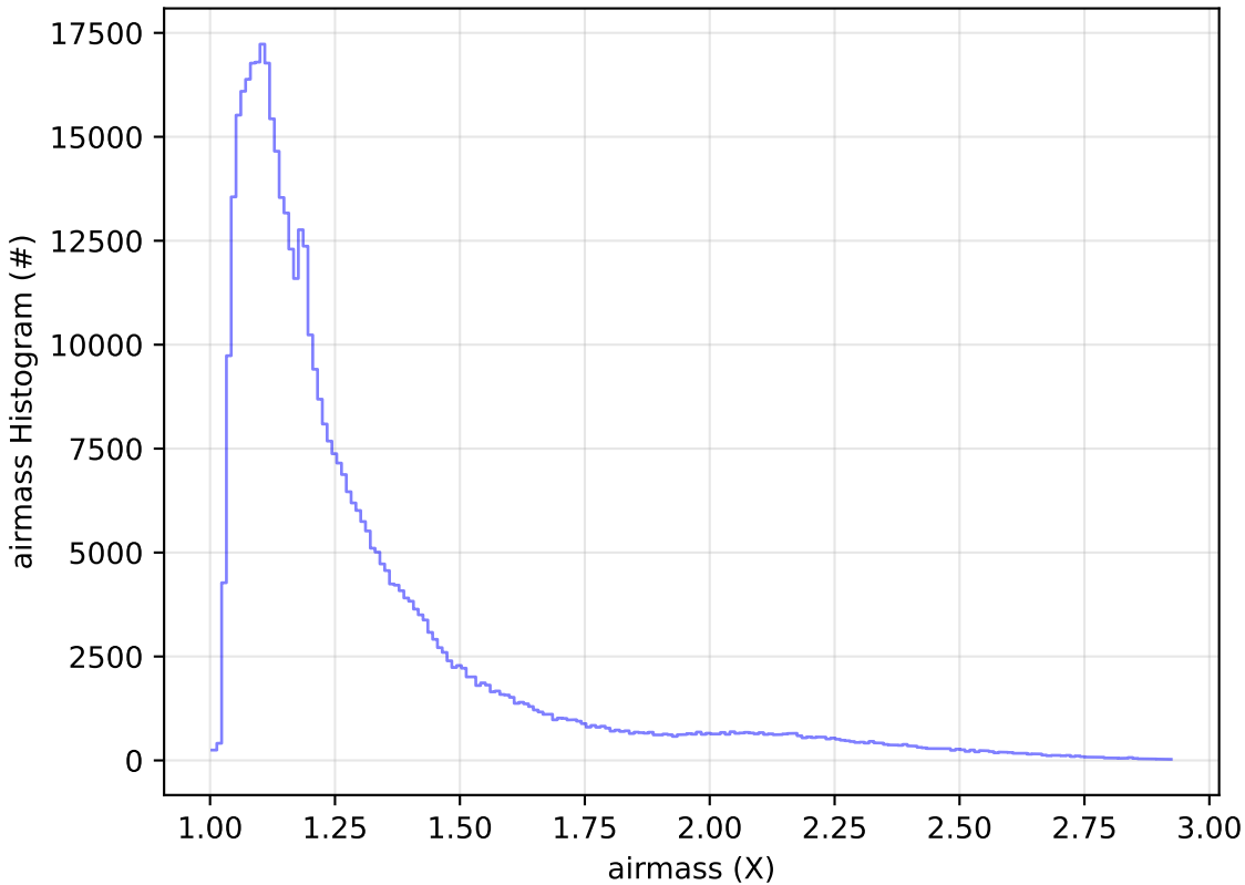
start_date_do-180v3.4_10yrs All sky i band: airmass Histogram
