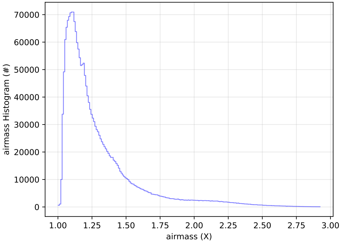
start_date_do-180v3.4_10yrs All sky all bands: airmass Histogram
