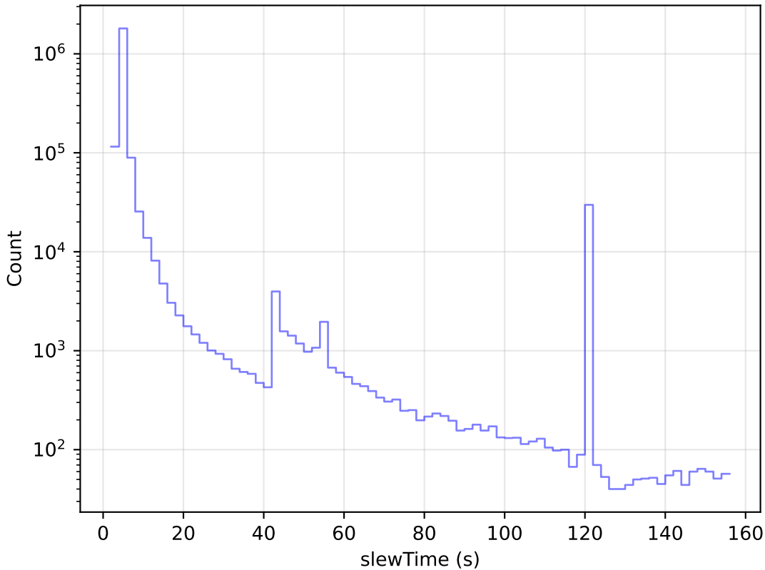
start_date_do-180v3.4_10yrs All visits: Slew Time Histogram
