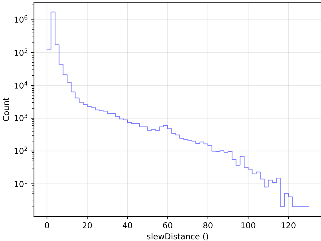
start_date_do-180v3.4_10yrs All visits: Slew Distance Histogram
