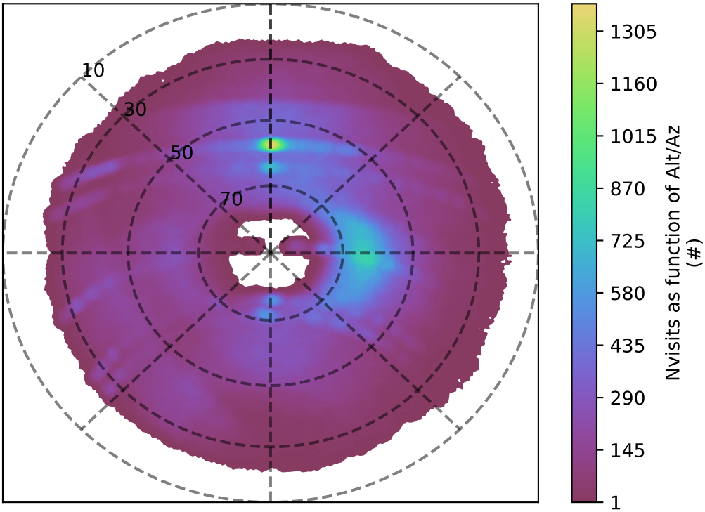
start_date_do-180v3.4_10yrs g band: Nvisits as function of Alt/Az
