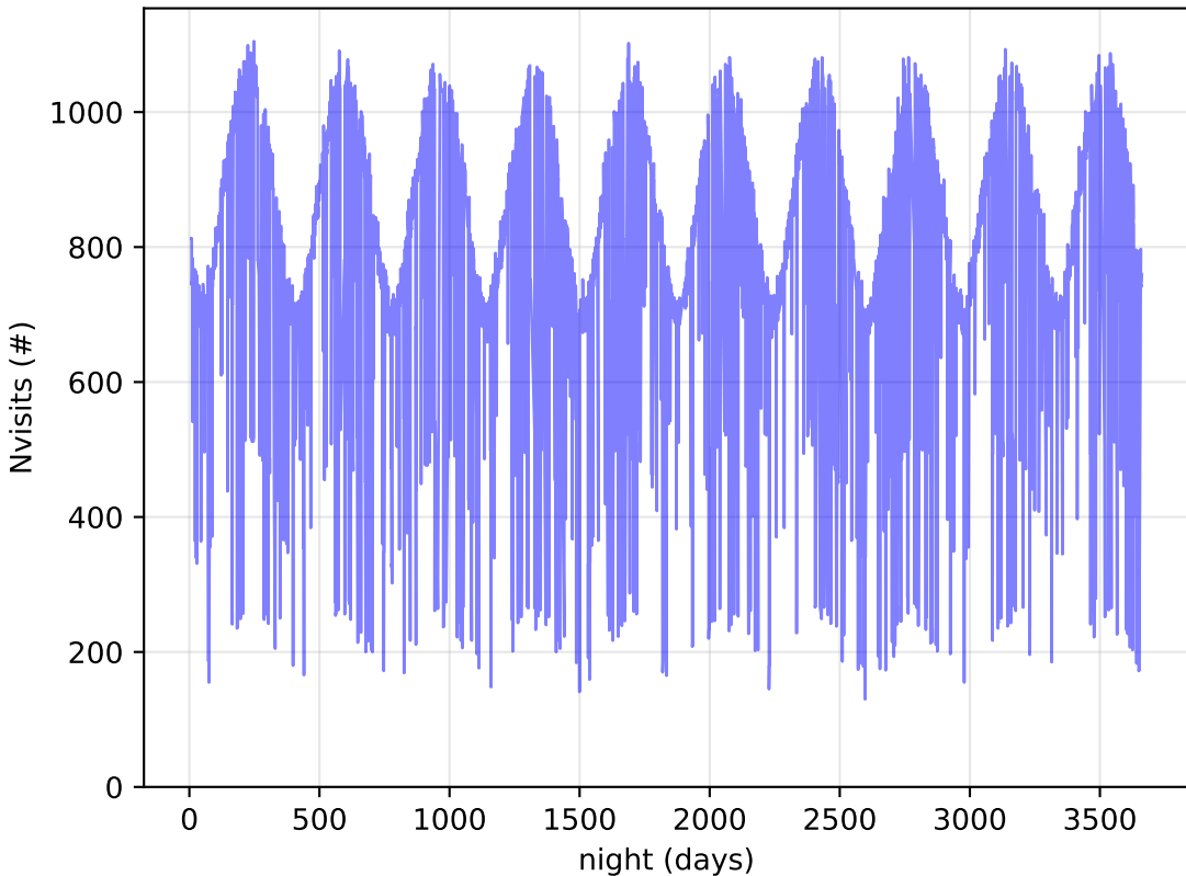
start_date_do-180v3.4_10yrs All visits: Nvisits
