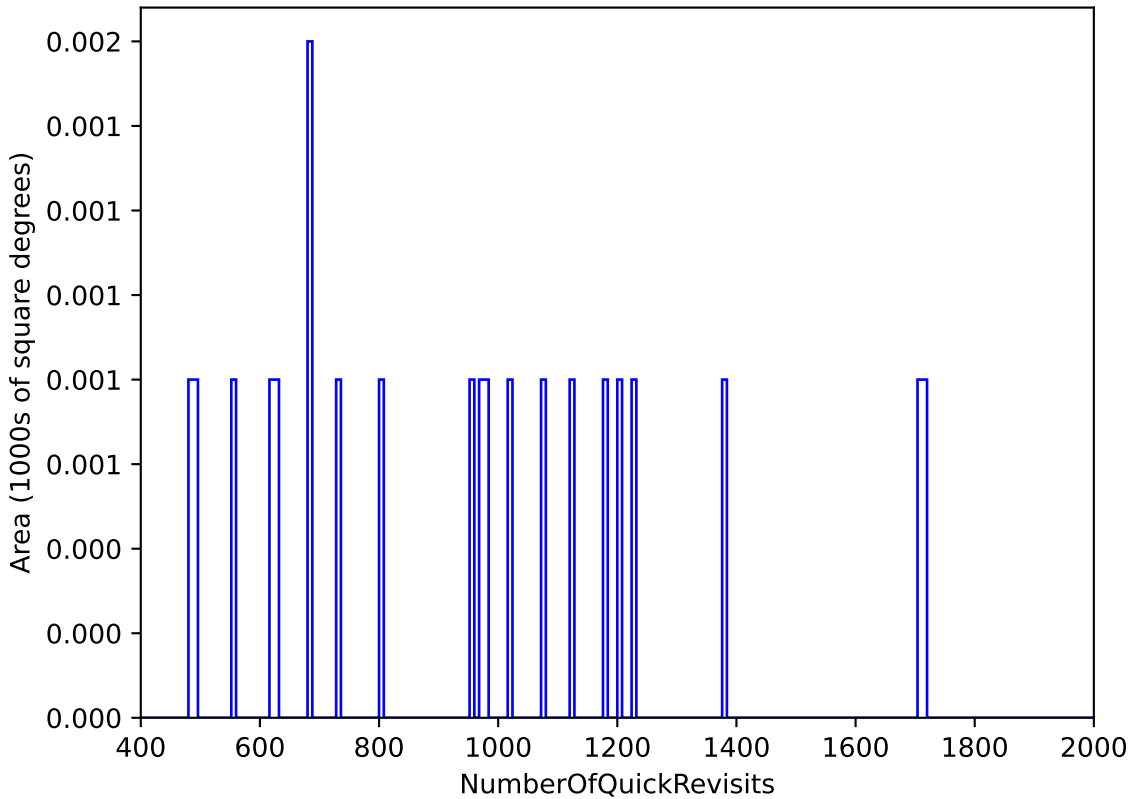
start_date_do-180v3.4_10yrs WFD: NumberOfQuickRevisits
