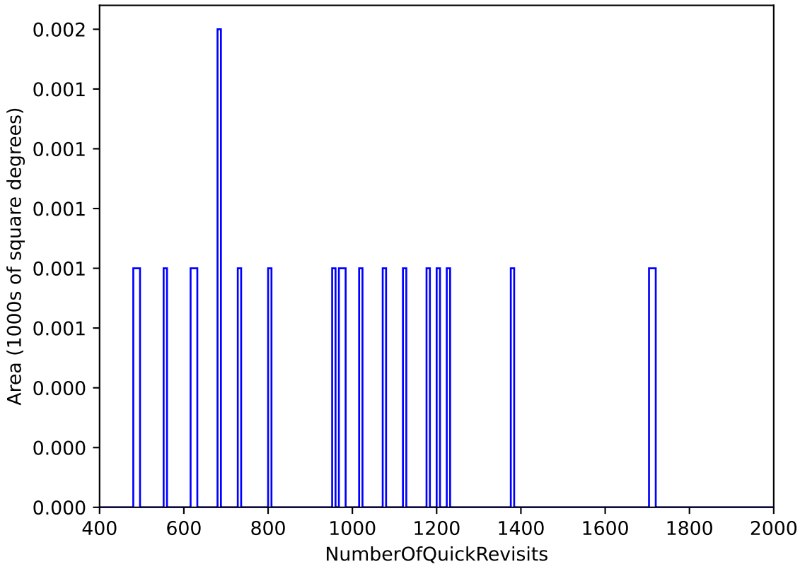
start_date_do-180v3.4_10yrs All sky: NumberOfQuickRevisits
