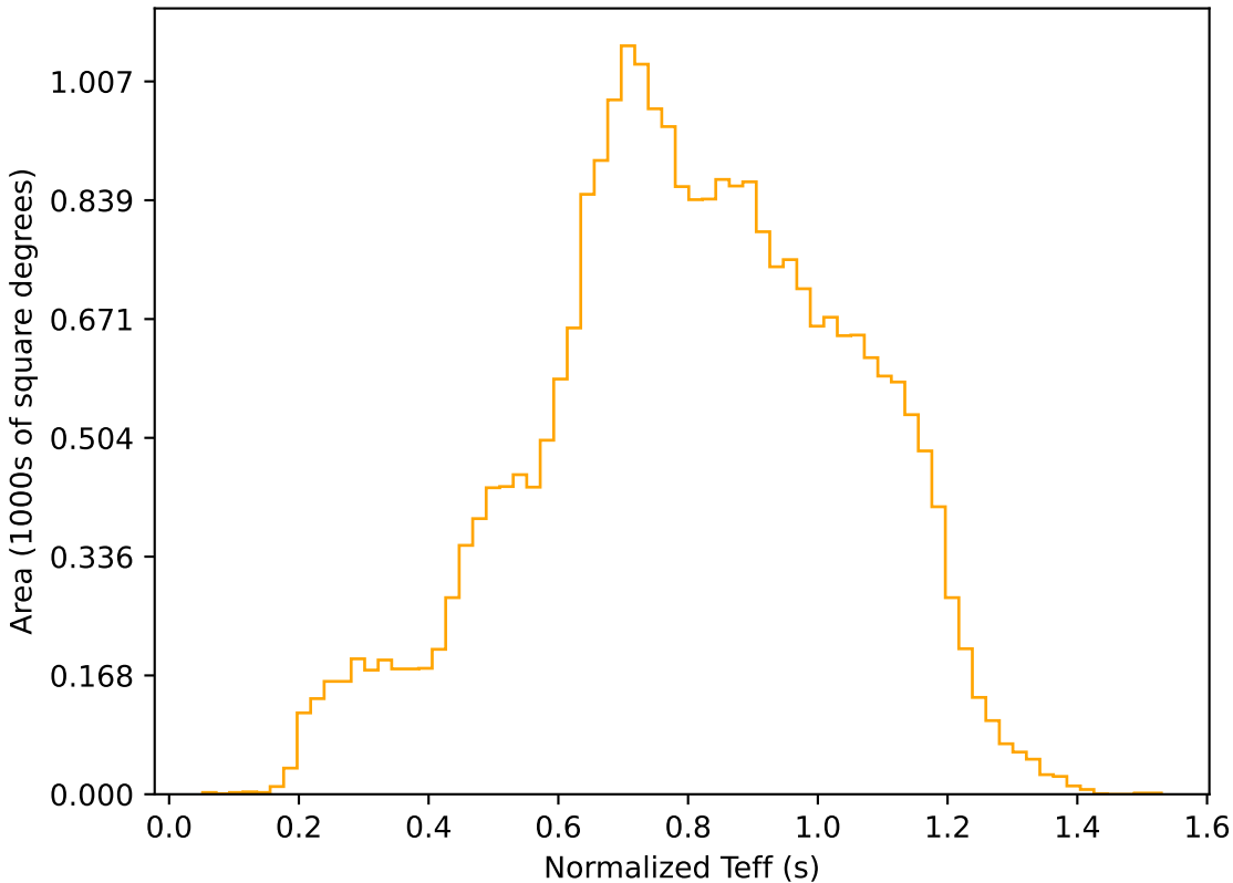
start_date_do-180v3.4_10yrs All sky r band: Normalized Teff
