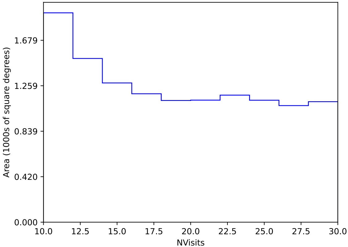
start_date_do-180v3.4_10yrs Yr 3-4 y band: NVisits
