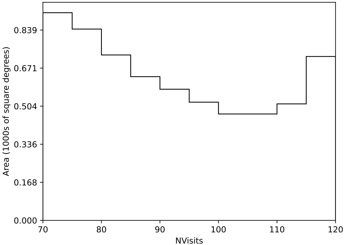
start_date_do-180v3.4_10yrs Yr 3-4 all bands: NVisits
