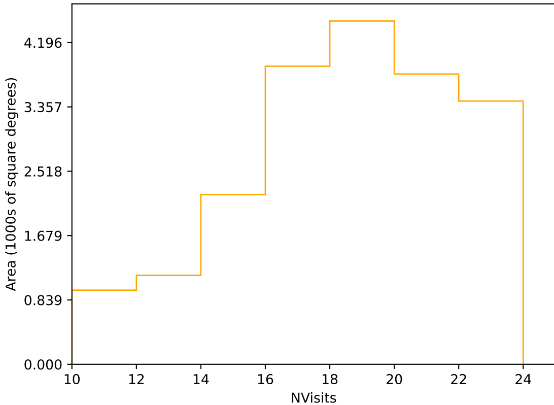
start_date_do-180v3.4_10yrs Yr 1 r band: NVisits
