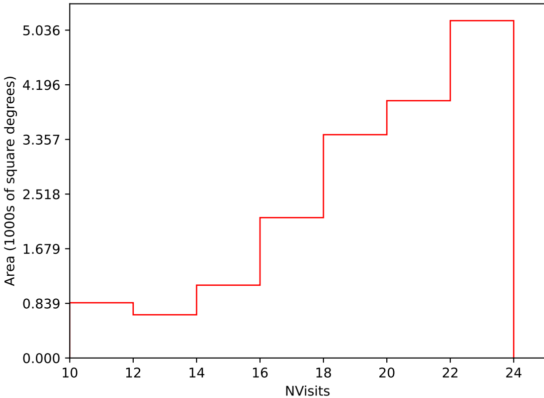
start_date_do-180v3.4_10yrs Yr 1 i band: NVisits
