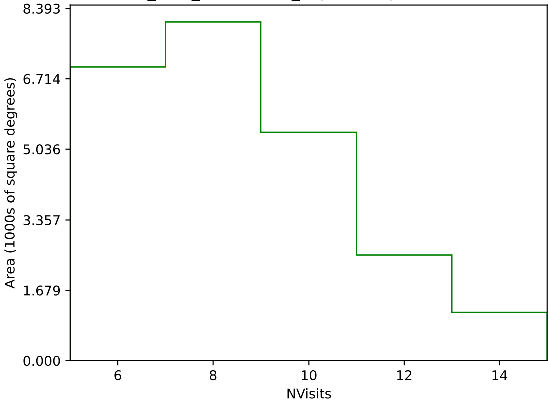
start_date_do-180v3.4_10yrs Yr 1 g band: NVisits
